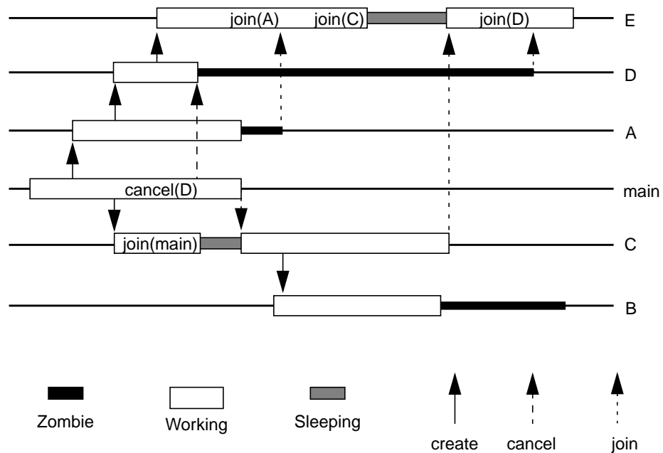
Figure 4-3 POSIX Thread Create and Join
